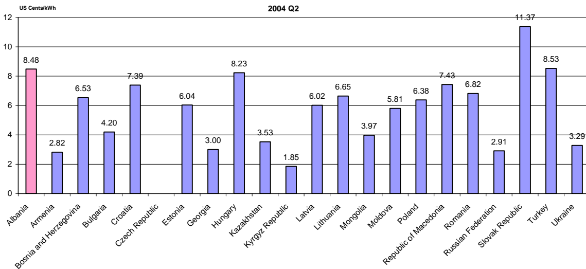
Average Electricity Price (Excluding Taxes) for Non-Residential Customers in ERRA Member Countries
